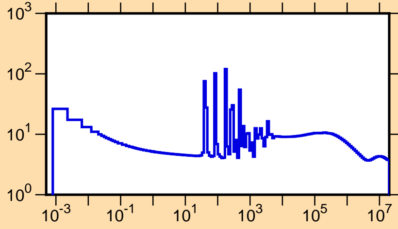
\sigma vs. E for ^{99}\text{Nb}(n,\text{tot.})
