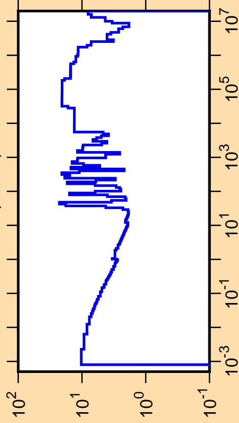
\Delta\sigma/\sigma vs. E for ^{99}\text{Nb}(n,\text{tot.})
