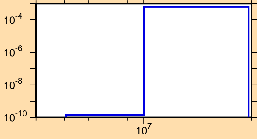
\sigma vs. E for ^{99}\text{Nb}(n,d)
