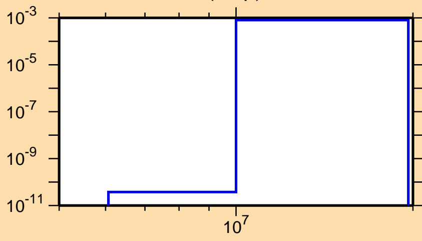
\sigma vs. E for ^{99}\text{Nb}(n,np)
