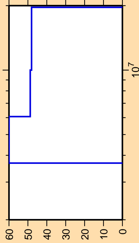
\Delta\sigma/\sigma vs. E for ^{99}\text{Nb}(n,p)
