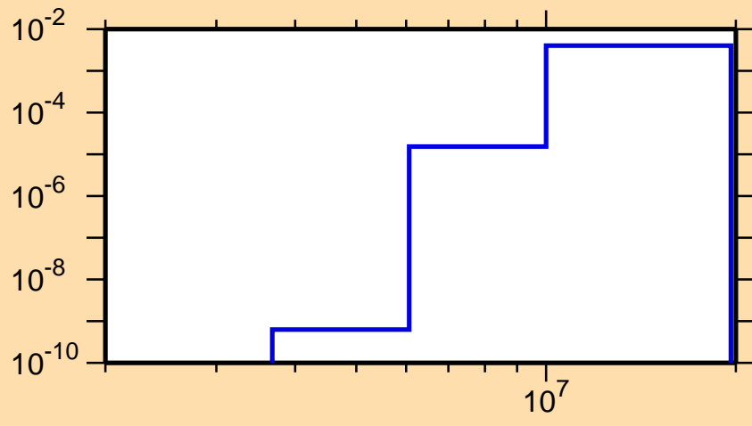
\sigma vs. E for ^{99}\text{Nb}(n,p)
