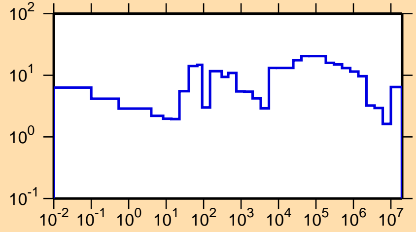
\Delta\sigma/\sigma vs. E for ^{99}\text{Nb}(n,\text{tot.})
