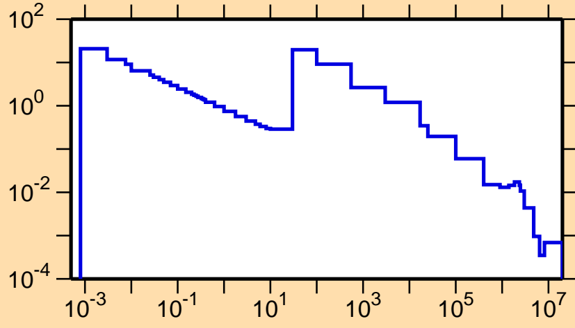
\sigma vs. E for ^{99}\text{Nb}(n,\gamma)
