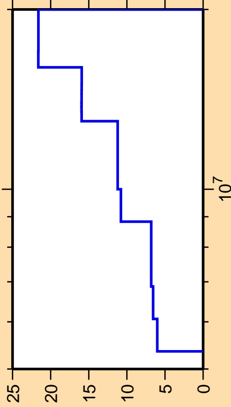
\Delta\sigma/\sigma vs. E for ^{102}\text{Nb}(n,p)
