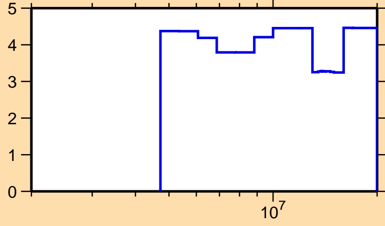
\Delta\sigma/\sigma vs. E for ^{102}\text{Nb}(n,\text{nonel.})
