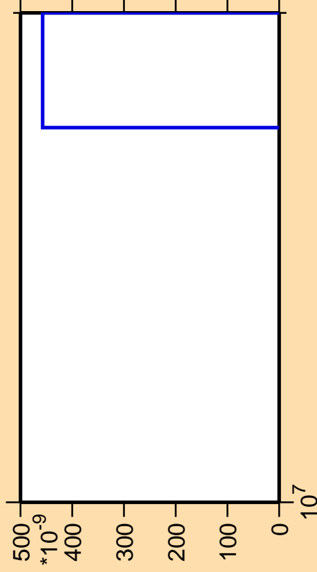
\Delta\sigma/\sigma vs. E for ^{102}\text{Nb} (mt 11)
