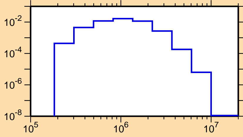
\sigma vs. E for ^{102}\text{Nb}(n,n_4)
