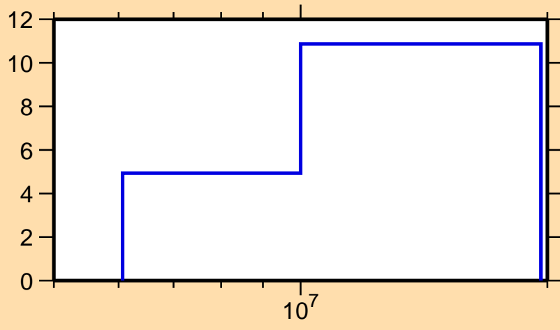
\Delta\sigma/\sigma vs. E for ^{103}\text{Nb}(n,el.)
