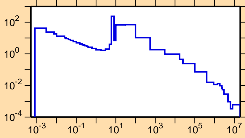
\sigma vs. E for ^{103}\text{Nb}(n,\gamma)
