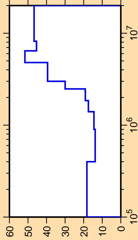
\Delta\sigma/\sigma vs. E for ^{103}\text{Nb}(n,n_3)
