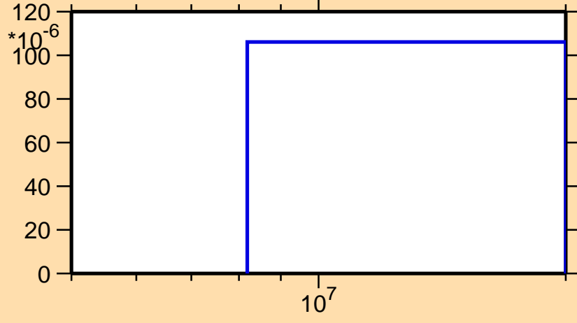
\sigma vs. E for ^{103}\text{Nb}(n,d)
