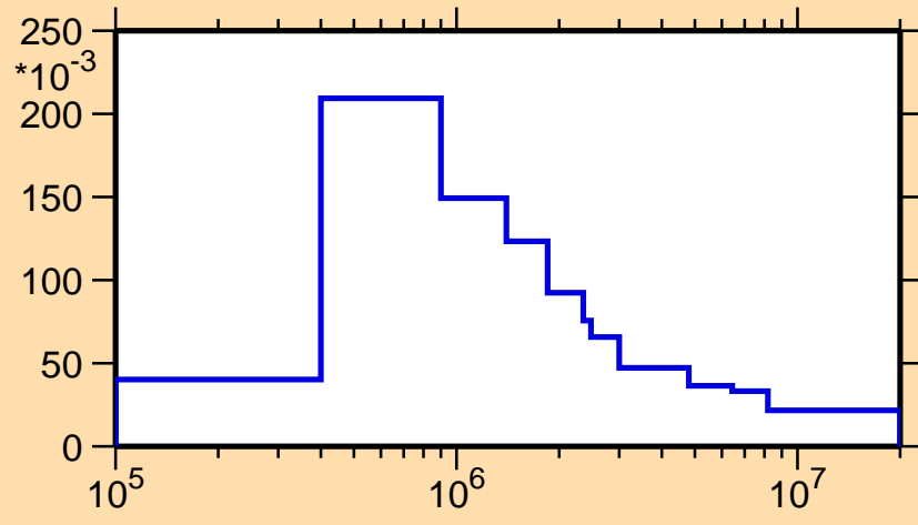
\sigma vs. E for ^{103}\text{Nb}(n,n_3)
