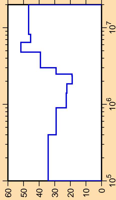
\Delta\sigma/\sigma vs. E for ^{103}\text{Nb}(n,n_4)
