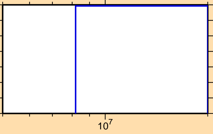
\sigma vs. E for ^{103}\text{Nb}(n,t)
