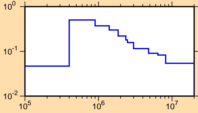
\sigma vs. E for ^{103}\text{Nb}(n,n_4)
