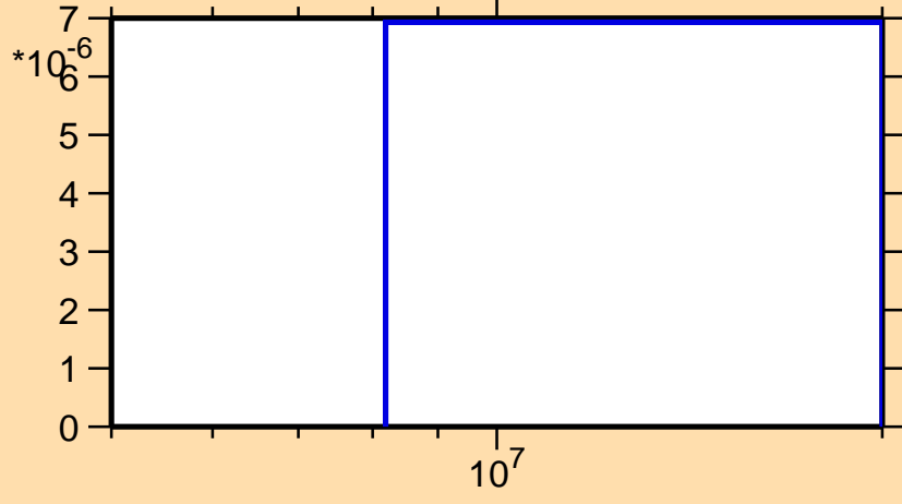
\sigma vs. E for ^{103}\text{Nb}(n,t)
