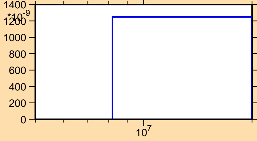
\sigma vs. E for ^{103}\text{Nb}(n,n\alpha)
