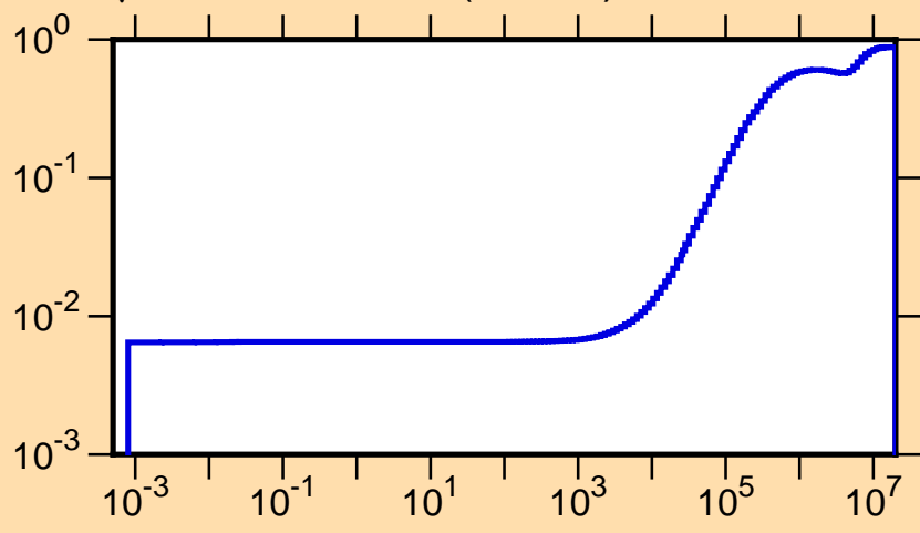
\mu vs. E for ^{104}\text{Nb}(\text{mt251})
