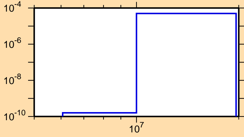
\sigma vs. E for ^{104}\text{Nb}(n,\alpha)
