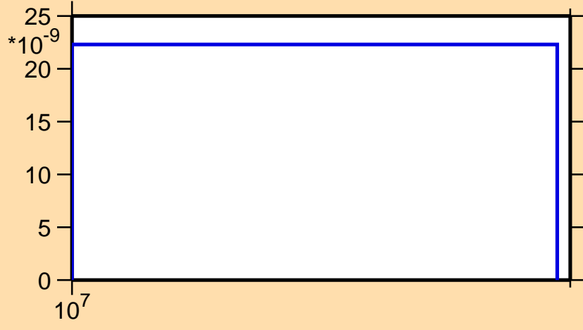
\sigma vs. E for ^{104}\text{Nb}(n,nt)
