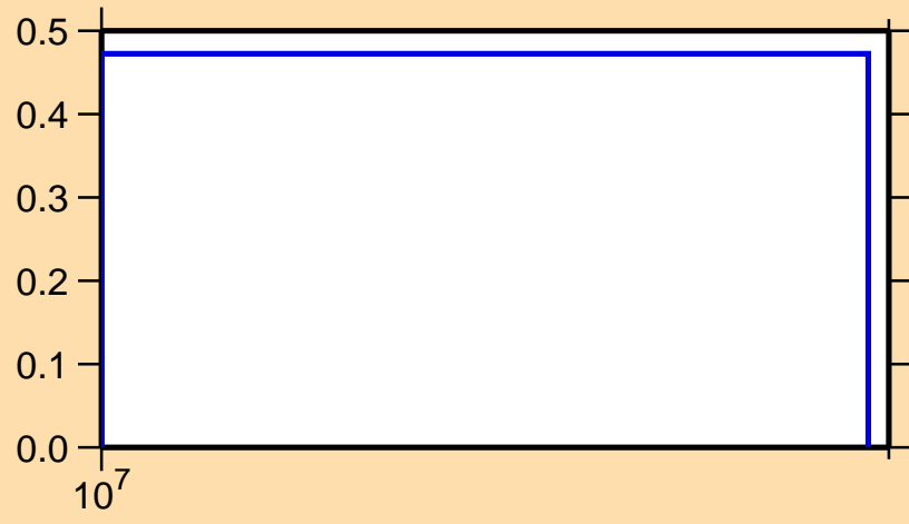
\sigma vs. E for ^{104}\text{Nb}(n,3n)
