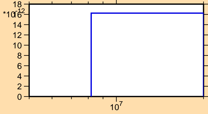
\sigma vs. E for ^{104}\text{Nb}(n,2n\alpha)
