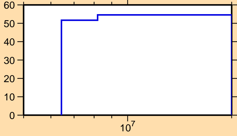
\Delta\sigma/\sigma vs. E for ^{104}\text{Nb}(n,\text{el.})
