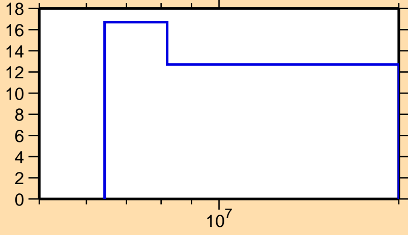
\Delta\sigma/\sigma vs. E for ^{104}\text{Nb}(n,\text{nonel.})
