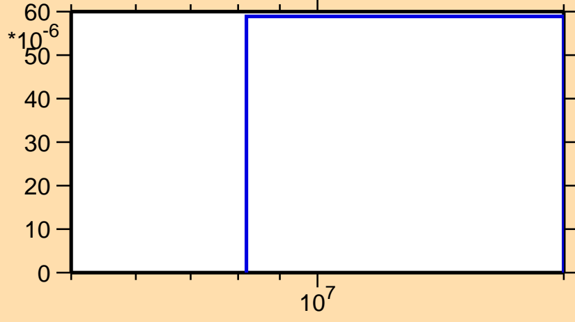
\sigma vs. E for ^{104}\text{Nb}(n,d)
