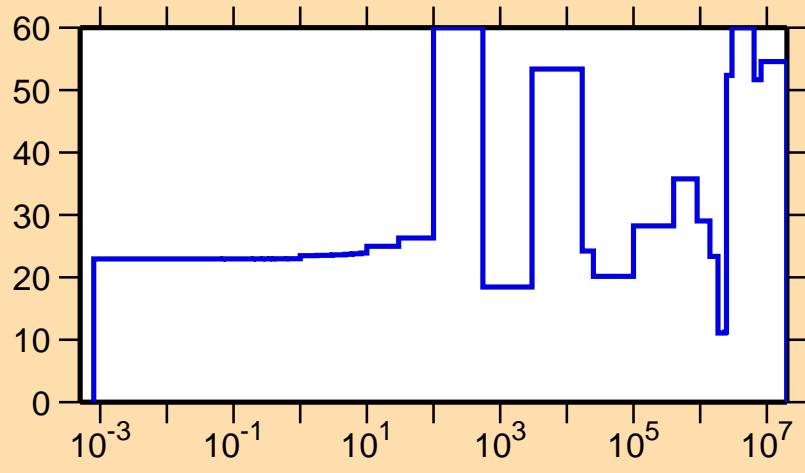
\Delta\sigma/\sigma vs. E for ^{104}\text{Nb}(n,\text{el.})
