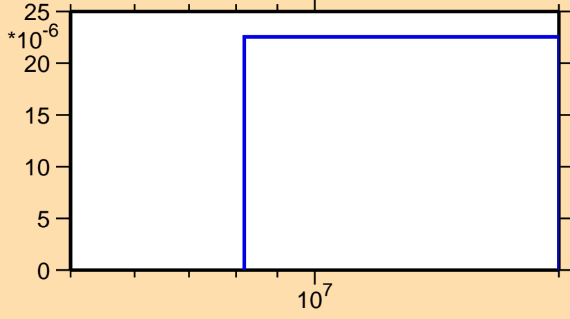
\sigma vs. E for ^{104}\text{Nb}(n,t)
