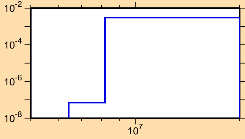
\sigma vs. E for ^{104}\text{Nb}(n,p)
