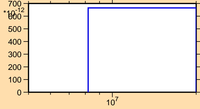
\sigma vs. E for ^{104}\text{Nb}(n,2np)
