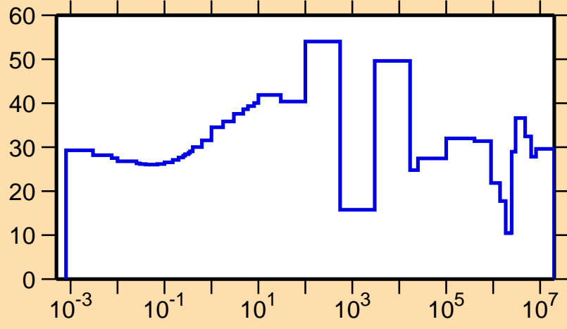
\Delta\sigma/\sigma vs. E for ^{104}\text{Nb}(n,\text{tot.})
