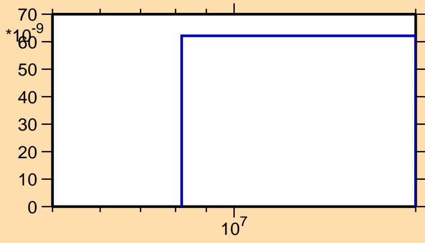
\sigma vs. E for ^{104}\text{Nb}(n,\text{nd})
