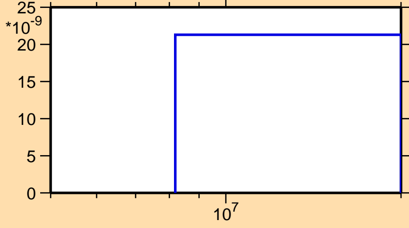
\sigma vs. E for ^{104}\text{Nb}(n,nt)
