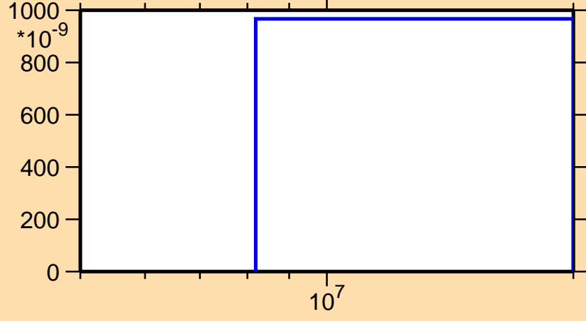
\sigma vs. E for ^{104}\text{Nb}(n,n\alpha)
