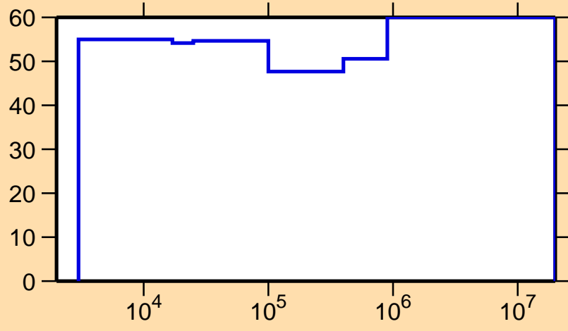
\Delta\sigma/\sigma vs. E for ^{104}\text{Nb}(n,n_1)
