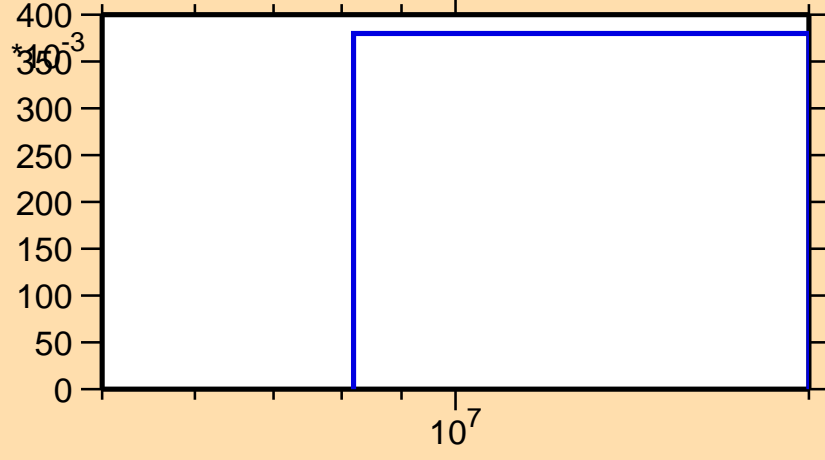
\sigma vs. E for ^{104}\text{Nb}(n,3n)
