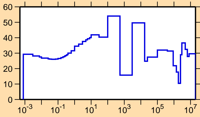
\Delta\sigma/\sigma vs. E for ^{104}\text{Nb}(n,\text{tot.})
