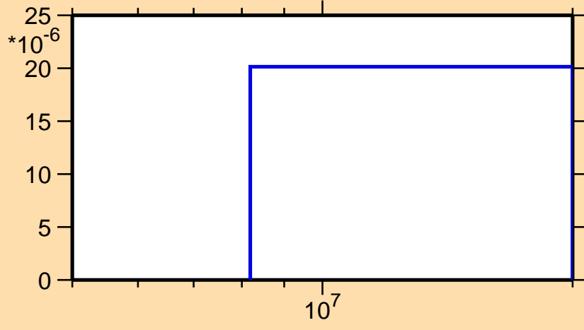
\sigma vs. E for ^{104}\text{Nb}(n,np)
