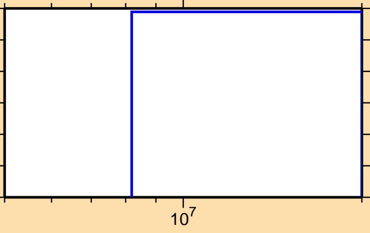
\sigma vs. E for ^{104}\text{Nb}(n,d)
