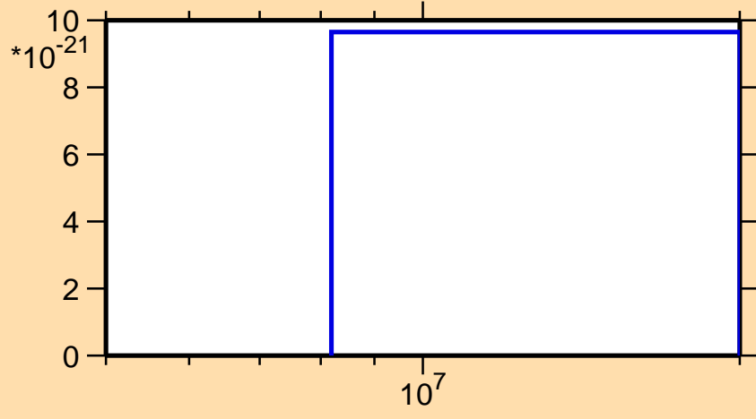
\sigma vs. E for ^{104}\text{Nb}(n,3n\alpha)
