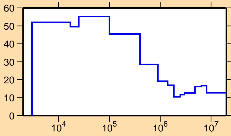
\Delta\sigma/\sigma vs. E for ^{104}\text{Nb}(n,\text{nonel.})
