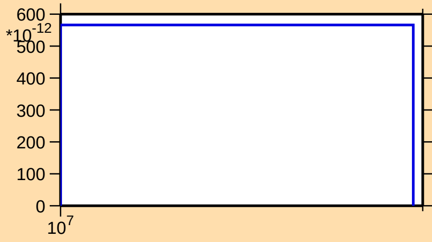
\sigma vs. E for ^{105}\text{Nb}(n,\text{nd})
