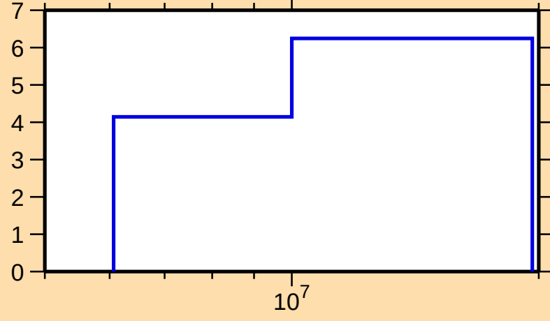
\Delta\sigma/\sigma vs. E for ^{105}\text{Nb}(n,\text{tot.})
