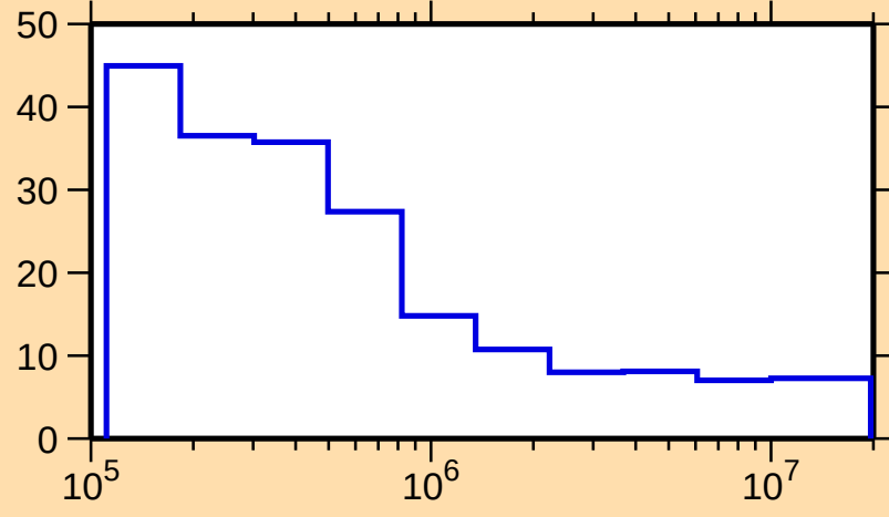
\Delta\sigma/\sigma vs. E for ^{105}\text{Nb}(n,\text{nonel.})
