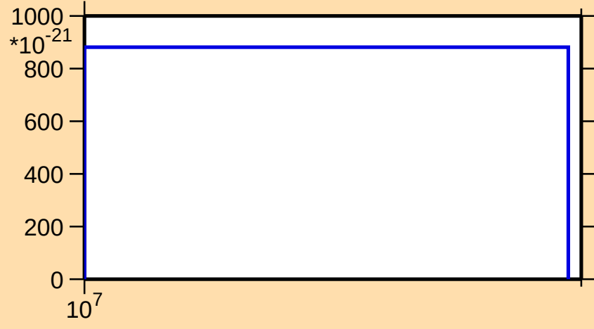
\sigma vs. E for ^{105}\text{Nb}(n,3n\alpha)
