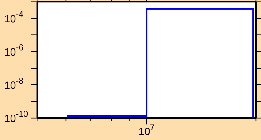
\sigma vs. E for ^{105}\text{Nb}(n,p)
