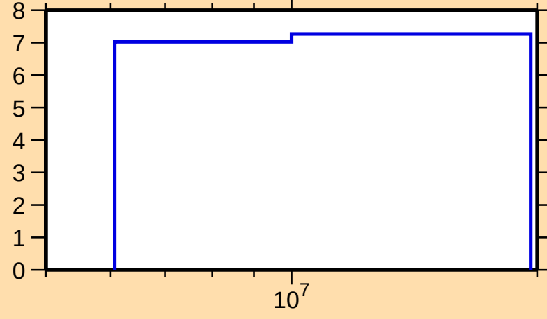
\Delta\sigma/\sigma vs. E for ^{105}\text{Nb}(n,\text{nonel.})
