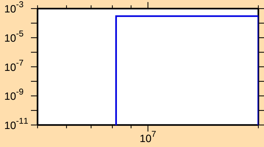
\sigma vs. E for ^{105}\text{Nb}(n,p)
