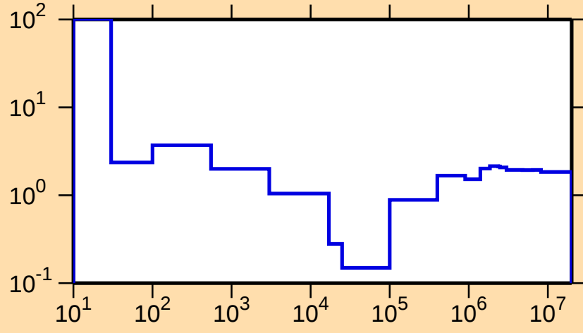
\sigma vs. E for ^{105}\text{Nb}(n,\text{nonel.})
