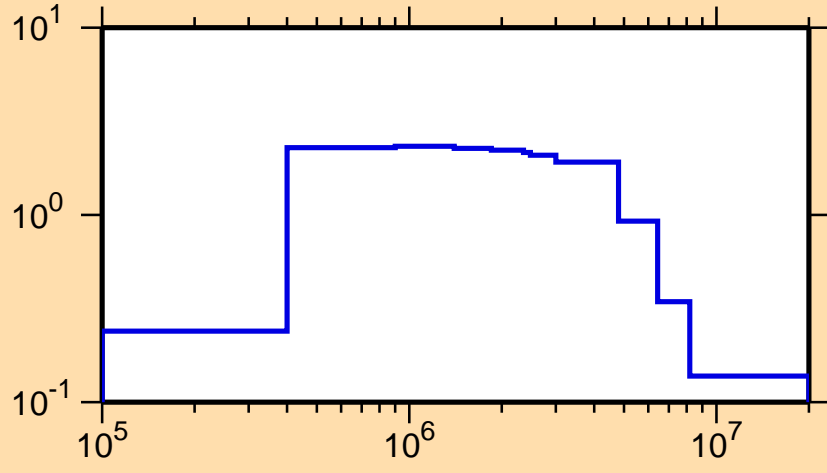
\sigma vs. E for ^{106}\text{Nb}(n,n\text{cont.})
