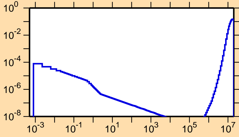
\sigma vs. E for ^{126}\text{Nd}(n,p\alpha)
