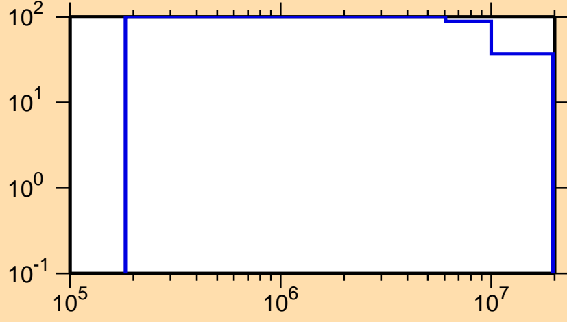
\Delta\sigma/\sigma vs. E for ^{126}\text{Nd}(n,n\text{cont.})
