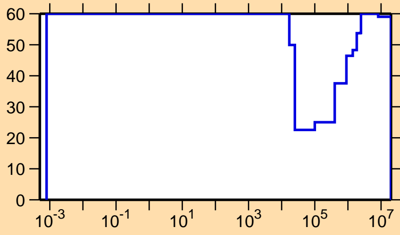
\Delta\sigma/\sigma vs. E for ^{126}\text{Nd}(n,p)
