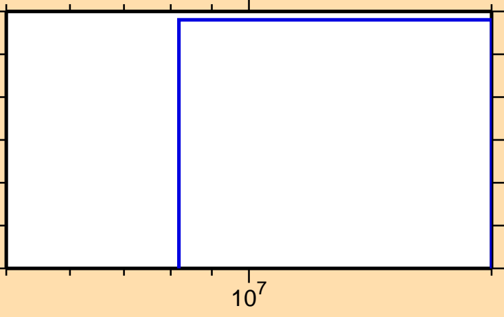
\sigma vs. E for ^{126}\text{Nd}(n,2n)
