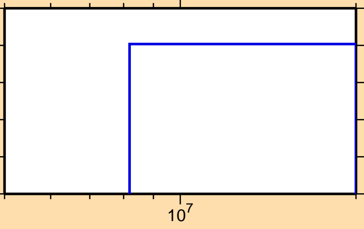
\sigma vs. E for ^{127}\text{Nd}(\text{mt117})
