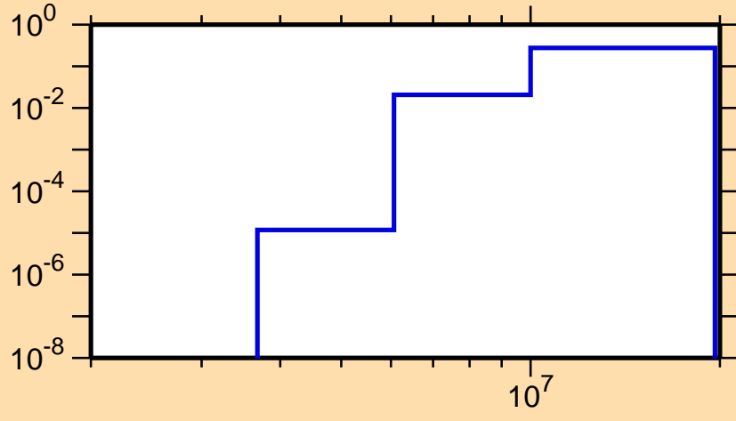
\sigma vs. E for ^{128}\text{Nd}(n,np)
