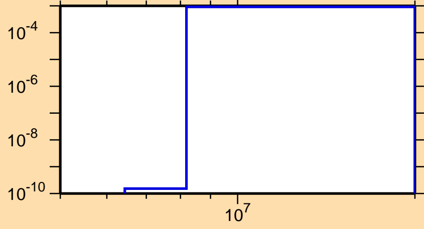
\sigma vs. E for ^{128}\text{Nd}(n,\text{pd})
