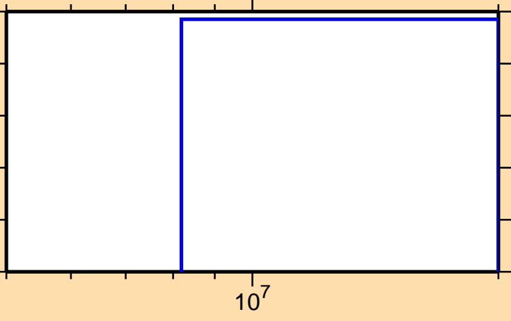
\sigma vs. E for ^{128}\text{Nd}(n,2np)
