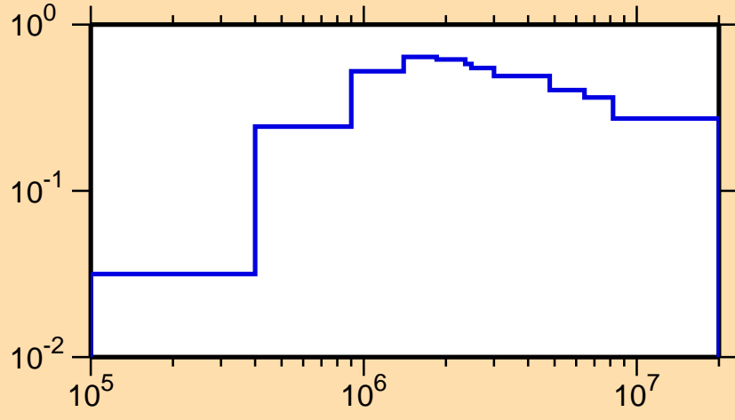
\sigma vs. E for ^{128}\text{Nd}(n,\text{inel.})
