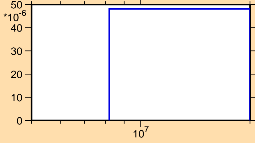
\sigma vs. E for ^{128}\text{Nd}(n,t)
