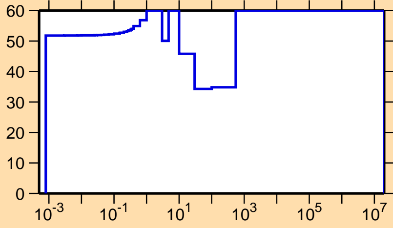
\Delta\sigma/\sigma vs. E for ^{128}\text{Nd}(n,\gamma)
