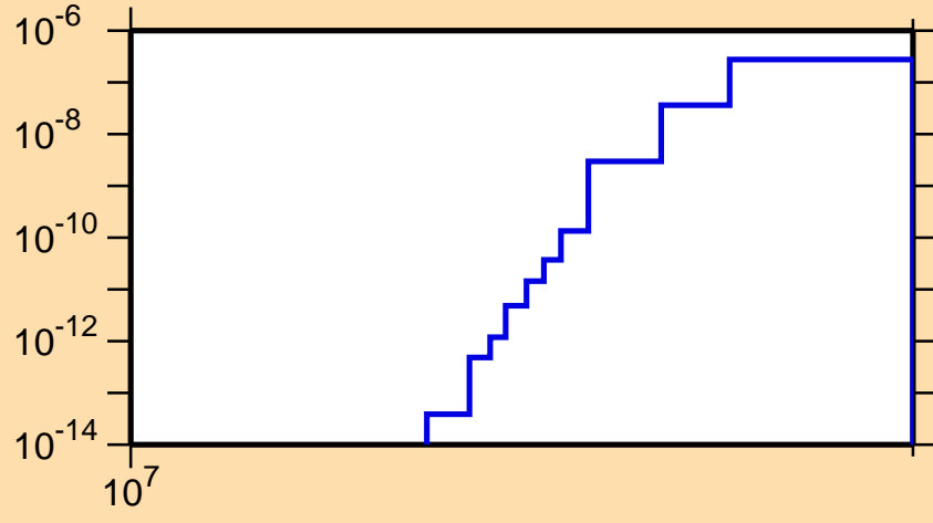
\sigma vs. E for ^{129}\text{Nd}(n,2n\alpha)
