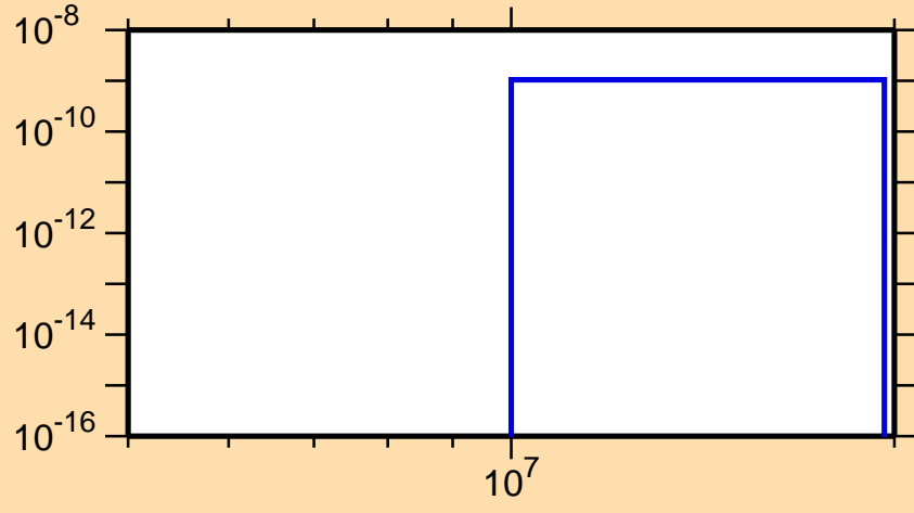
\sigma vs. E for ^{129}\text{Nd}(\text{mt117})
