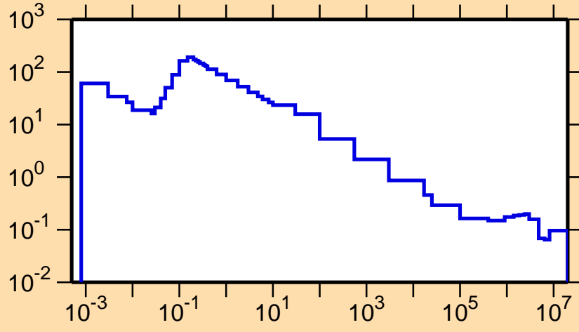
\sigma vs. E for ^{129}\text{Nd}(n,\alpha)
