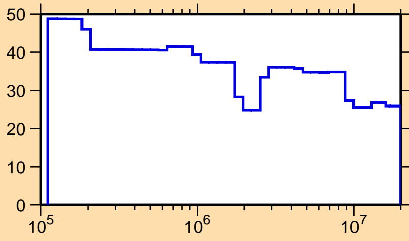
\Delta\sigma/\sigma vs. E for ^{131}\text{Nd}(n,\text{nonel.})
