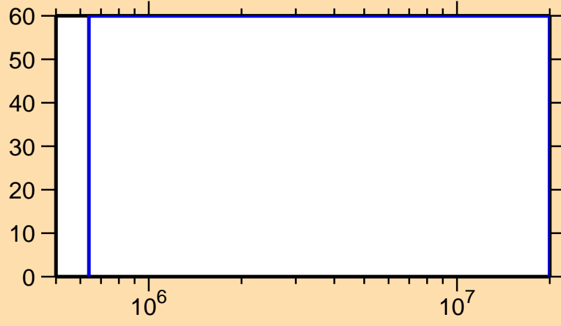
\Delta\sigma/\sigma vs. E for ^{131}\text{Nd}(n,n\text{cont.})
