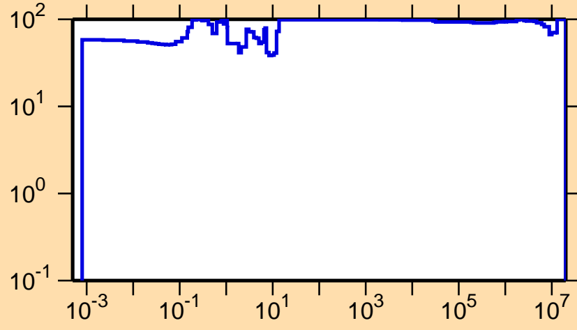
\Delta\sigma/\sigma vs. E for ^{131}\text{Nd}(n,\gamma)
