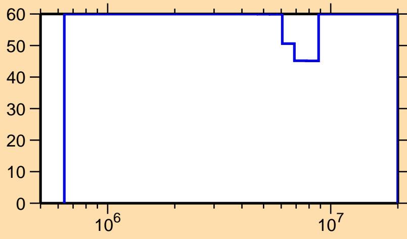
\Delta\sigma/\sigma vs. E for ^{131}\text{Nd}(n,\text{inel.})
