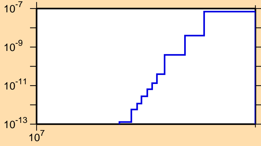
\sigma vs. E for ^{131}\text{Nd}(\text{mt } 34)
