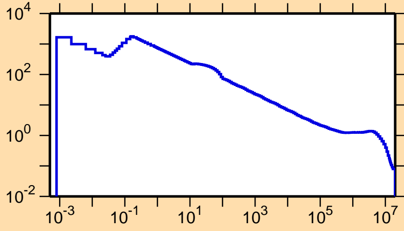
\sigma vs. E for ^{131}\text{Nd}(n,p)
