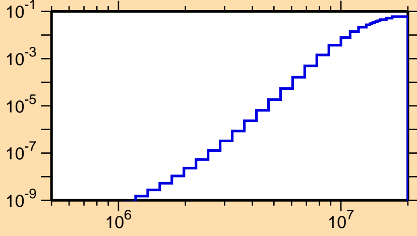
\sigma vs. E for ^{131}\text{Nd}(n,p\alpha)
