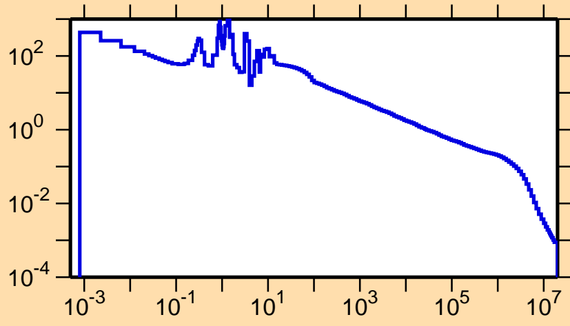
\sigma vs. E for ^{131}\text{Nd}(n,\gamma)
