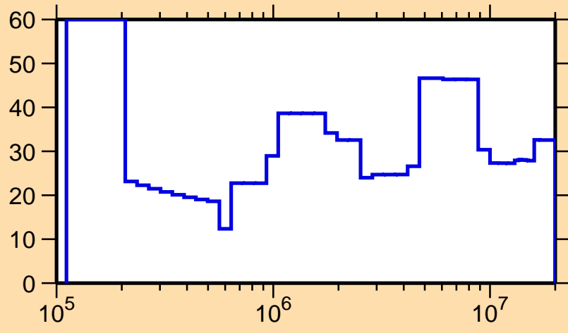
\Delta\sigma/\sigma vs. E for ^{131}\text{Nd}(n,\text{el.})
