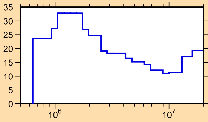
\Delta\sigma/\sigma vs. E for ^{131}\text{Nd}(n,\text{tot.})
