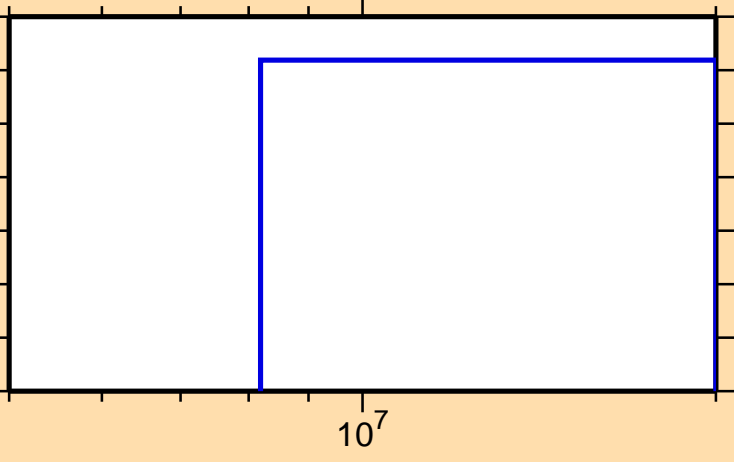
\sigma vs. E for ^{131}\text{Nd}(n,\text{pt})
