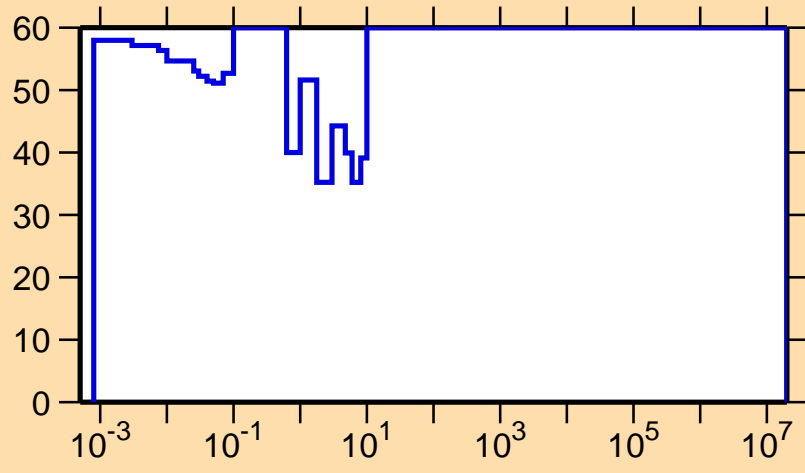
\Delta\sigma/\sigma vs. E for ^{131}\text{Nd}(n,\gamma)
