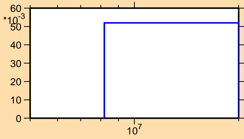
\sigma vs. E for ^{131}\text{Nd}(n,2n)
