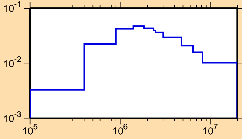
\sigma vs. E for ^{131}\text{Nd}(n,n_4)
