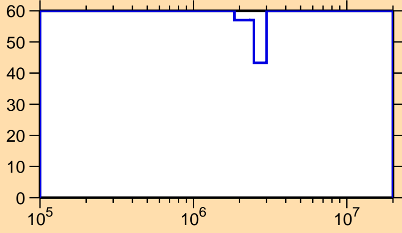
\Delta\sigma/\sigma vs. E for ^{131}\text{Nd}(n,n_1)
