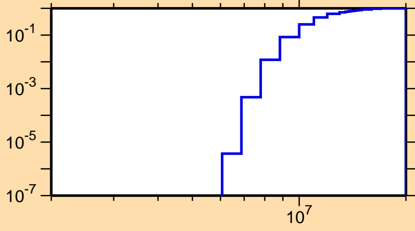
\sigma vs. E for ^{132}\text{Nd}(n,np)
