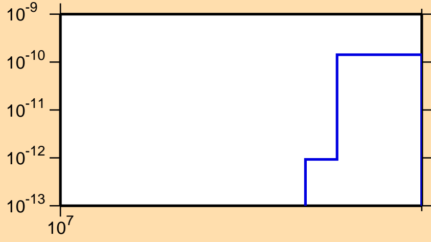
\sigma vs. E for ^{132}\text{Nd} (mt 34)
