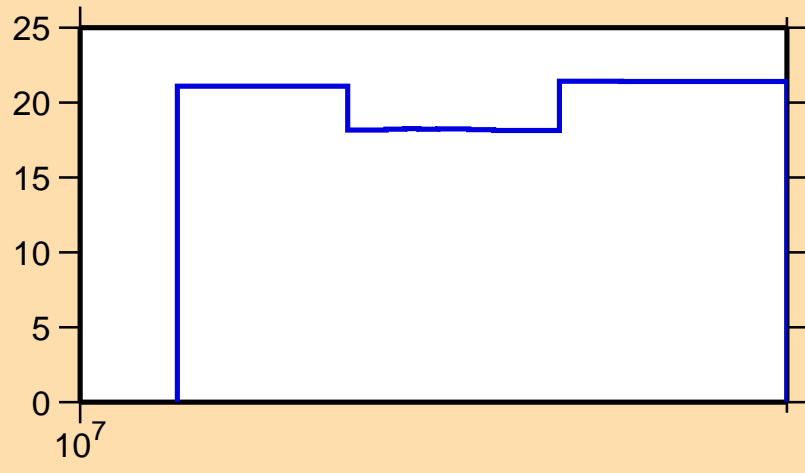
\Delta\sigma/\sigma vs. E for ^{132}\text{Nd}(n,\text{nonel.})
