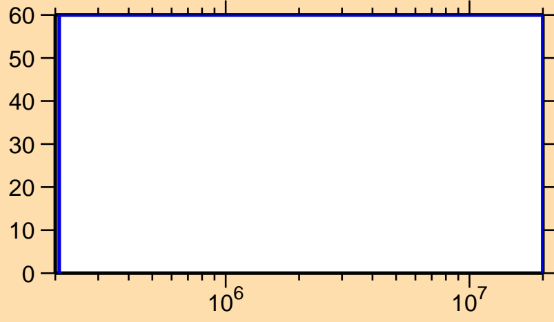
\Delta\sigma/\sigma vs. E for ^{132}\text{Nd}(n,n_1)
