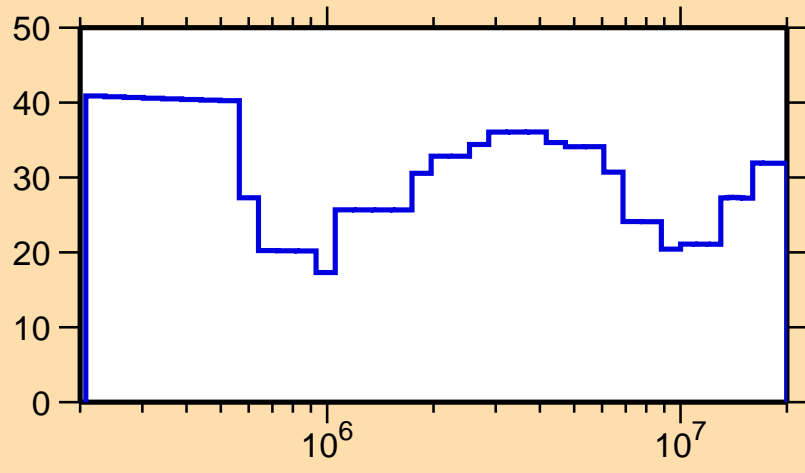
\Delta\sigma/\sigma vs. E for ^{132}\text{Nd}(n,\text{el.})
