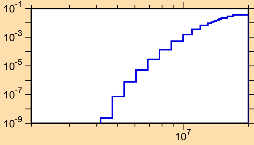
\sigma vs. E for ^{132}\text{Nd}(n,n\alpha)
