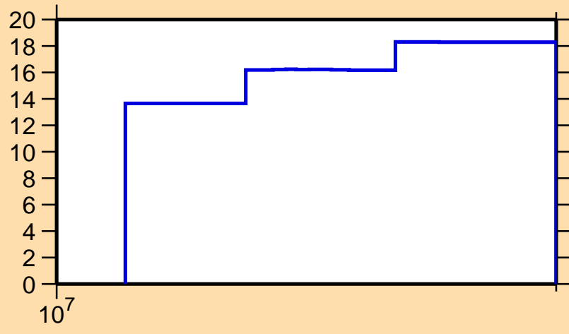
\Delta\sigma/\sigma vs. E for ^{132}\text{Nd}(n,\text{tot.})
