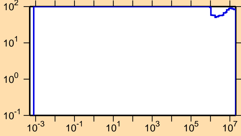
\Delta\sigma/\sigma vs. E for ^{132}\text{Nd}(n,p)
