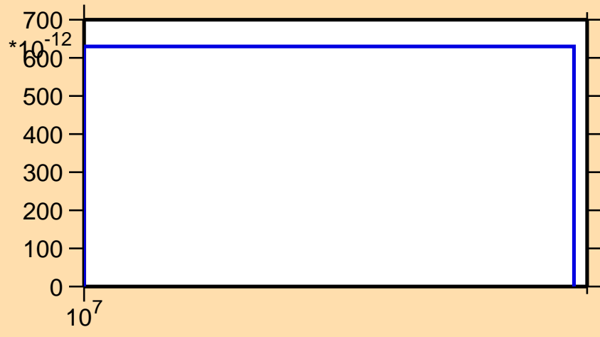
\sigma vs. E for ^{132}\text{Nd}(n,\text{nd})
