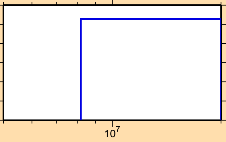
\sigma vs. E for ^{132}\text{Nd}(\text{mt117})
