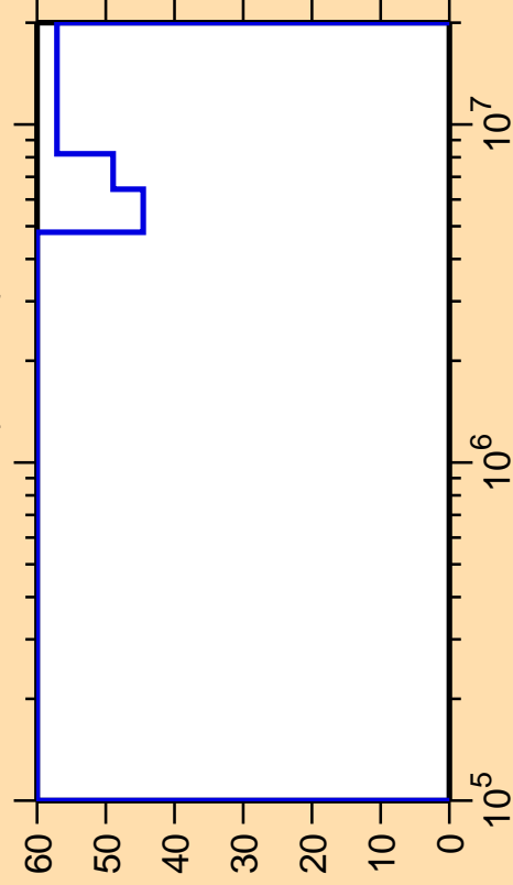
\Delta\sigma/\sigma vs. E for ^{132}\text{Nd}(n,\text{inel.})
