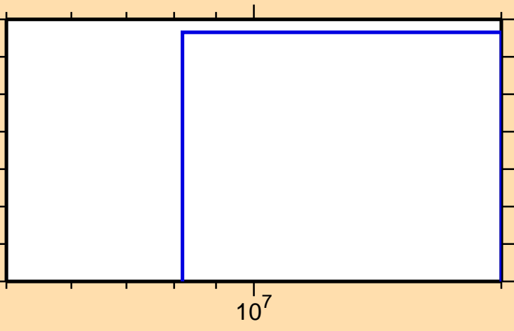
\sigma vs. E for ^{132}\text{Nd}(n,\text{nd})
