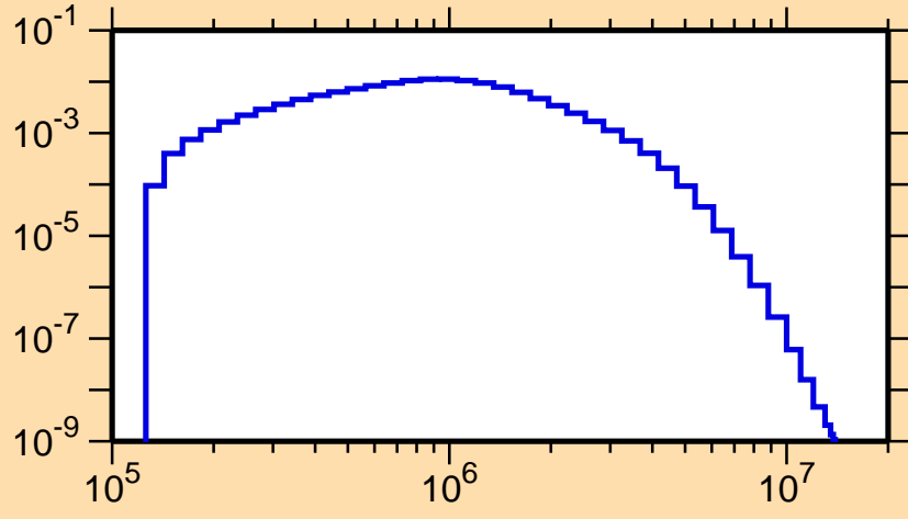
\sigma vs. E for ^{133}\text{Nd}(n,n_1)
