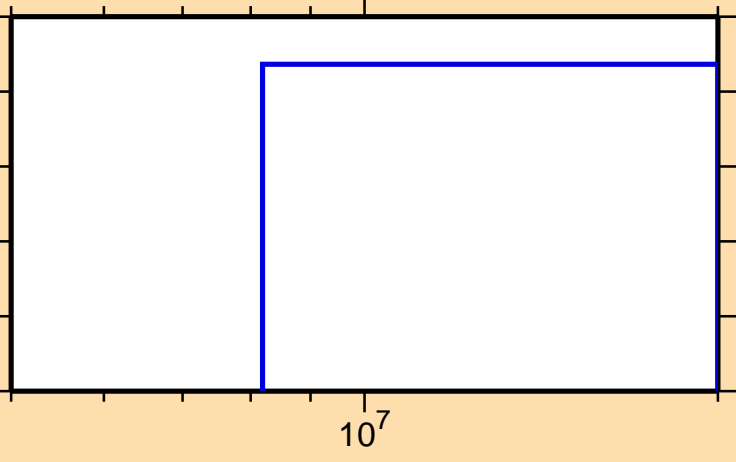
\sigma vs. E for ^{133}\text{Nd}(n,\text{pd})
