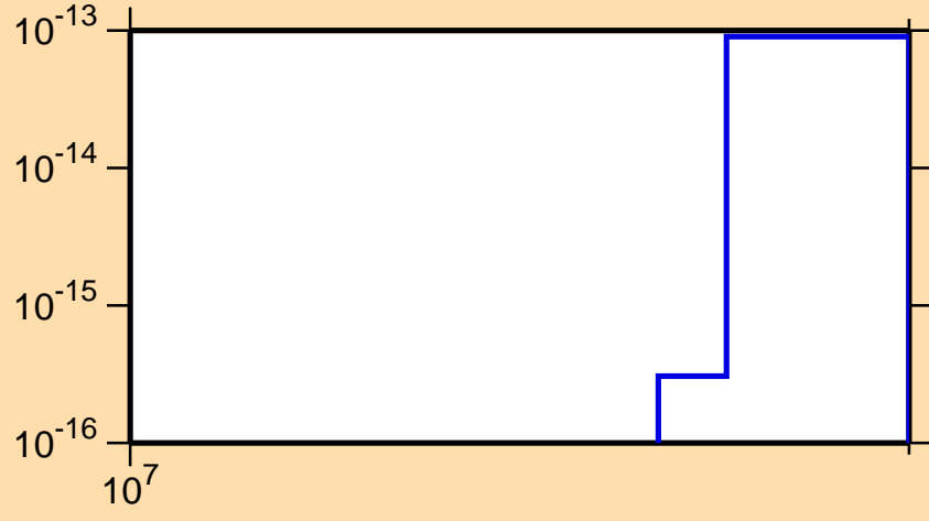
\sigma vs. E for ^{134}\text{Nd}(n,nt)
