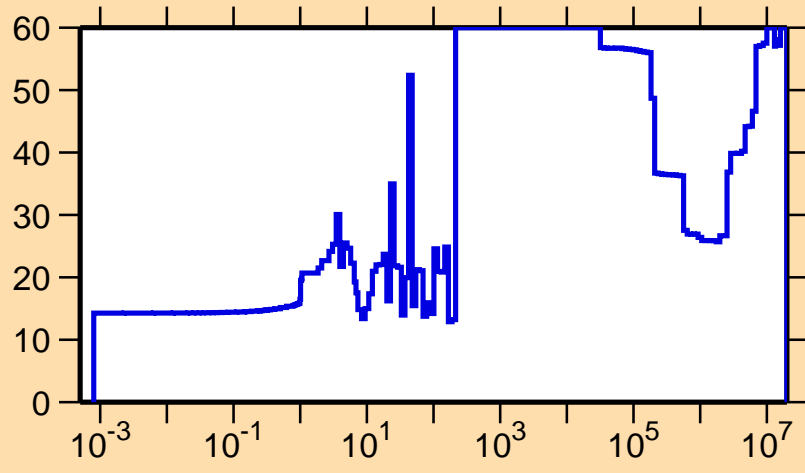
\Delta\sigma/\sigma vs. E for ^{134}\text{Nd}(n,\gamma)
