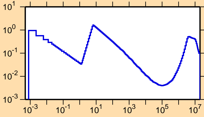
\sigma vs. E for ^{134}\text{Nd}(n,p)
