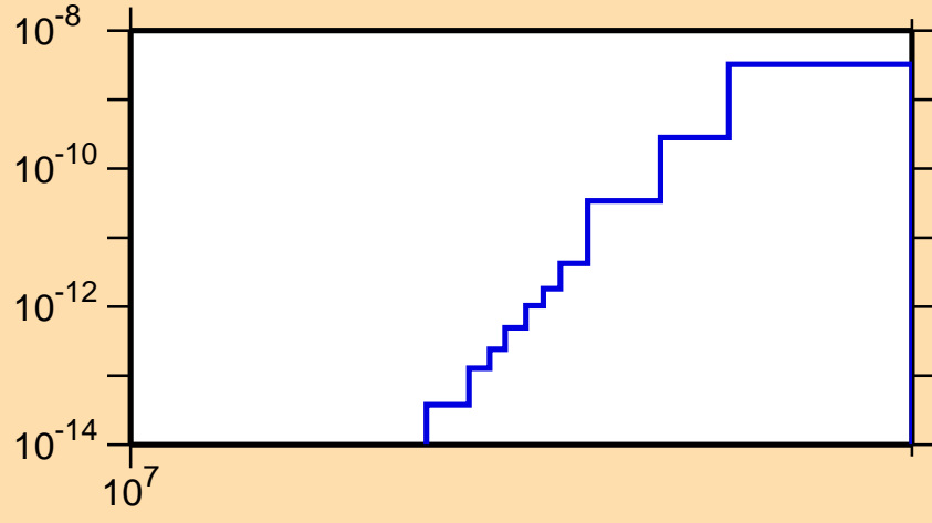
\sigma vs. E for ^{134}\text{Nd}(\text{mt117})
