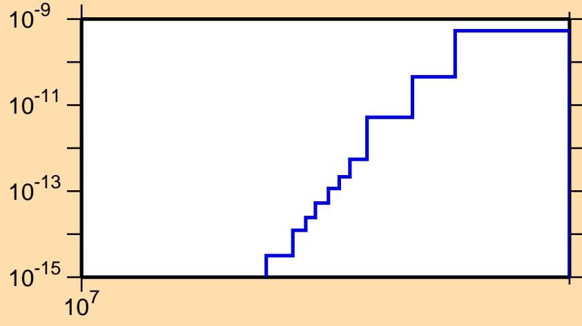
\sigma vs. E for ^{135}\text{Nd}(\text{mt117})
