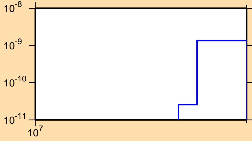
\sigma vs. E for ^{135}\text{Nd} (mt 34)
