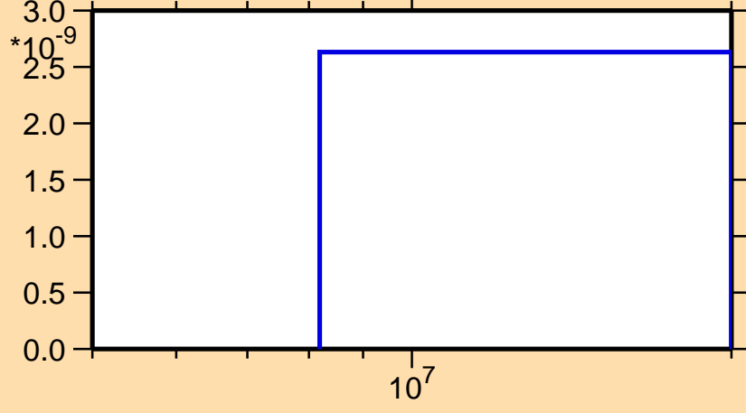
\sigma vs. E for ^{135}\text{Nd}(n,\text{pt})
