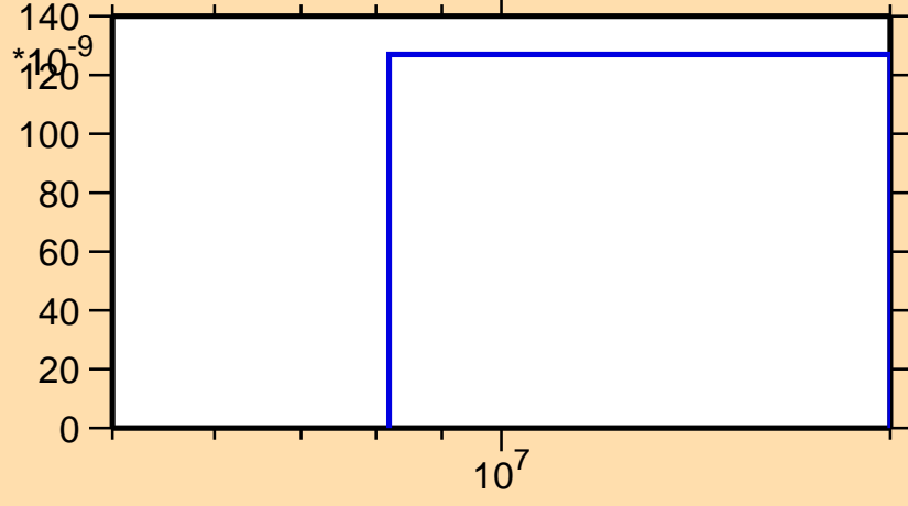
\sigma vs. E for ^{135}\text{Nd}(n,\text{nd})
