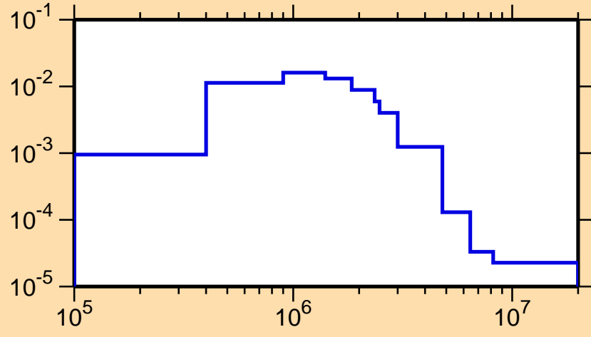
\sigma vs. E for ^{135}\text{Nd}(n,n_2)
