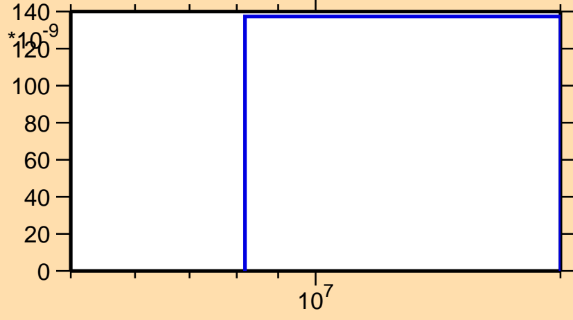
\sigma vs. E for ^{135}\text{Nd}(n,\text{pd})
