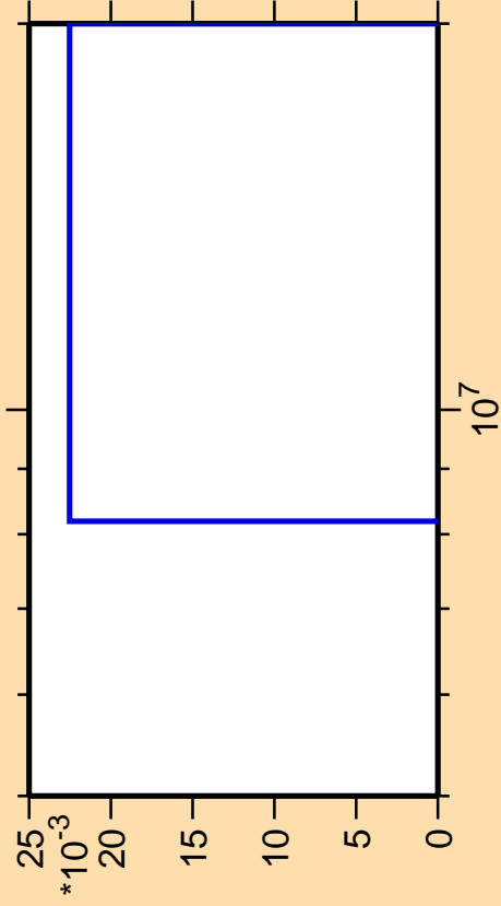
\Delta\sigma/\sigma vs. E for ^{135}\text{Nd}(n,nt)
