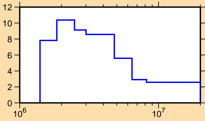
\Delta\sigma/\sigma vs. E for ^{135}\text{Nd}(n,\text{tot.})
