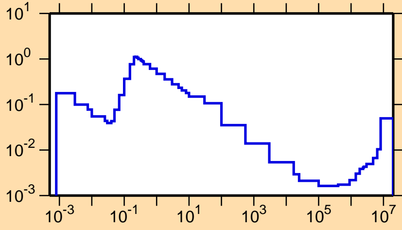
\sigma vs. E for ^{135}\text{Nd}(n,\alpha)
