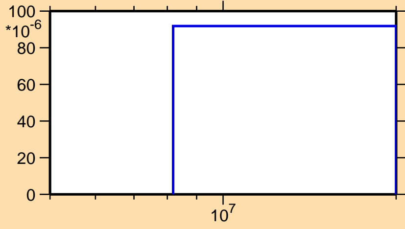
\sigma vs. E for ^{135}\text{Nd}(n,t)
