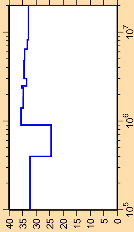
\Delta\sigma/\sigma vs. E for ^{135}\text{Nd}(n,n_2)
