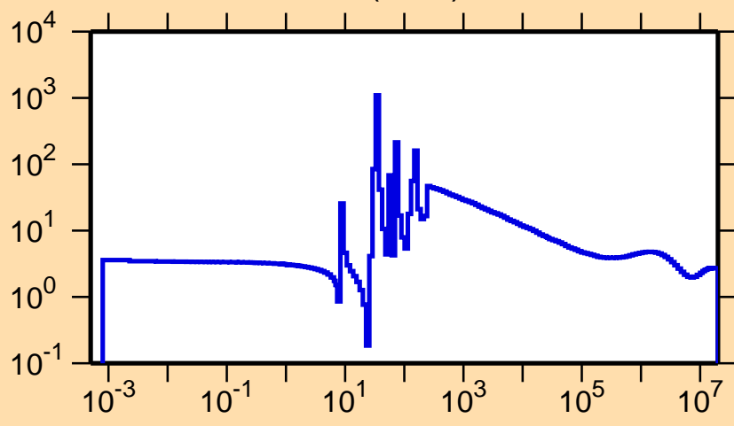
\sigma vs. E for ^{136}\text{Nd}(n,\text{el.})
