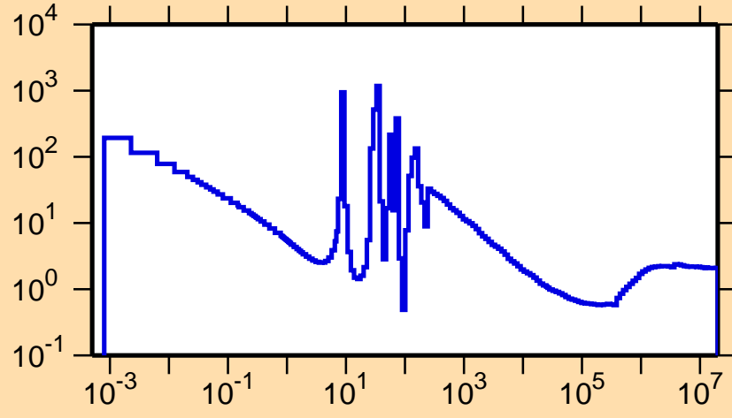
\sigma vs. E for ^{136}\text{Nd}(n,\text{nonel.})
