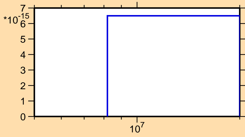
\sigma vs. E for ^{136}\text{Nd}(\text{mt } 34)
