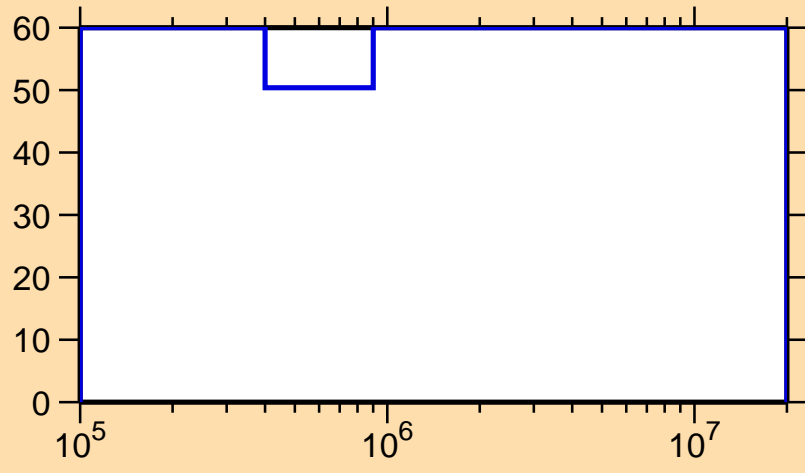
\Delta\sigma/\sigma vs. E for ^{136}\text{Nd}(n,n_1)
