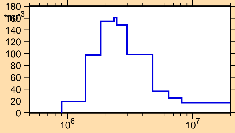
\sigma vs. E for ^{136}\text{Nd}(n,n_3)
