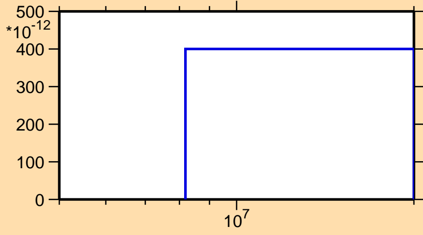
\sigma vs. E for ^{136}\text{Nd}(n,3n)
