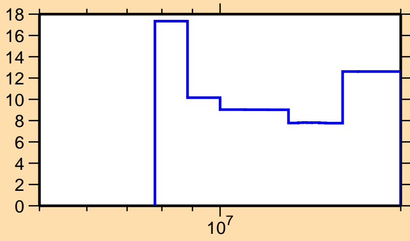
\Delta\sigma/\sigma vs. E for ^{139}\text{Nd}(n,\text{el.})
