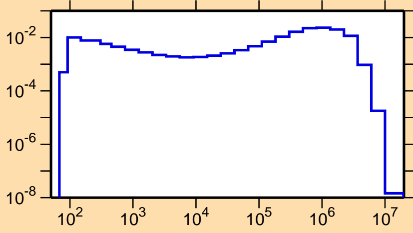
\sigma vs. E for ^{139}\text{Nd}(n,n_1)
