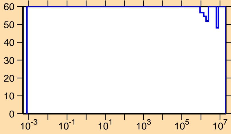
\Delta\sigma/\sigma vs. E for ^{139}\text{Nd}(n,p)
