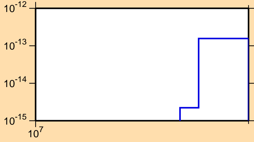
\sigma vs. E for ^{141}\text{Nd}(\text{mt117})
