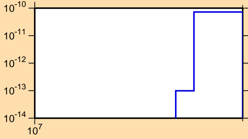
\sigma vs. E for ^{141}\text{Nd}(n,\text{pt})
