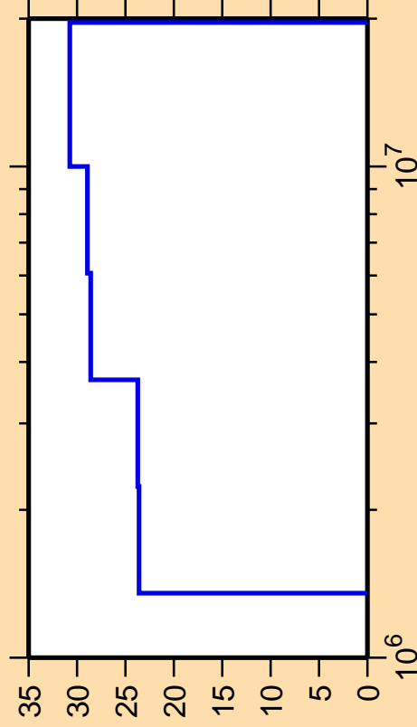
\Delta\sigma/\sigma vs. E for ^{142}\text{Nd}(n,n_1)
