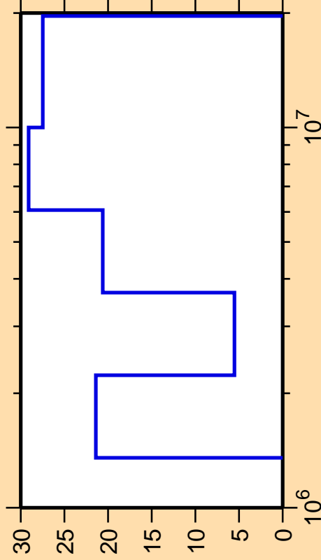
\Delta\sigma/\sigma vs. E for ^{142}\text{Nd}(n,n_2)
