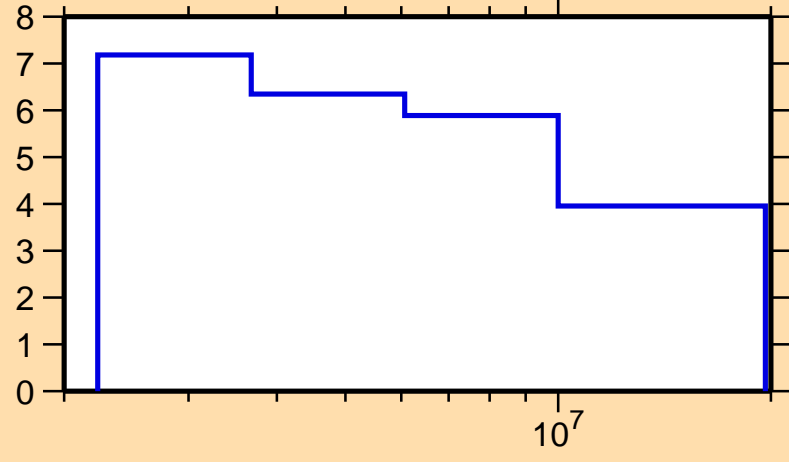
\Delta\sigma/\sigma vs. E for ^{142}\text{Nd}(n,n\text{onel.})
