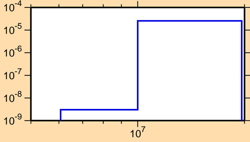
\sigma vs. E for ^{142}\text{Nd}(n,n\alpha)
