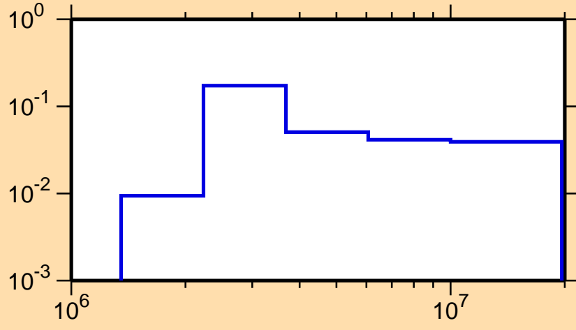
\sigma vs. E for ^{142}\text{Nd}(n,n_2)
