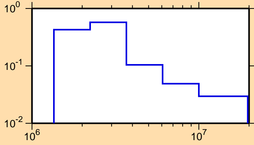
\sigma vs. E for ^{142}\text{Nd}(n,n_1)
