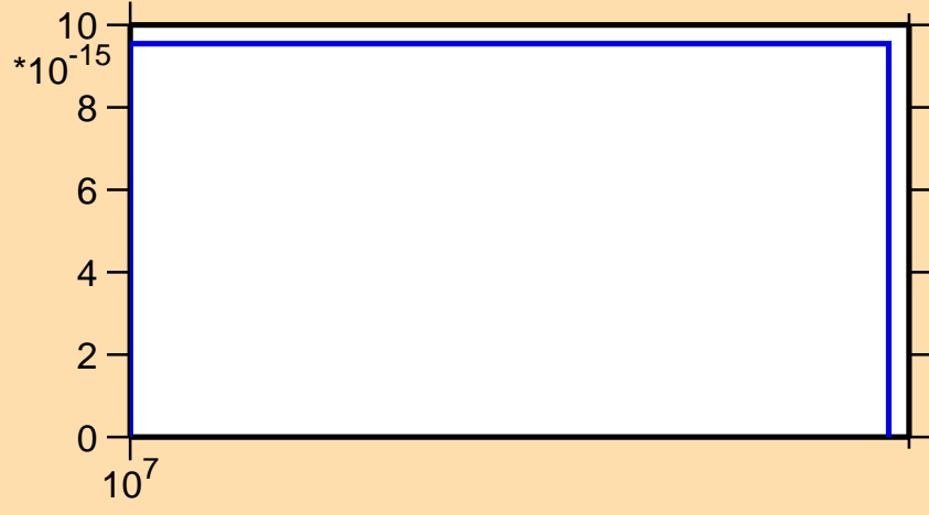
\sigma vs. E for ^{142}\text{Nd}(n,nt)
