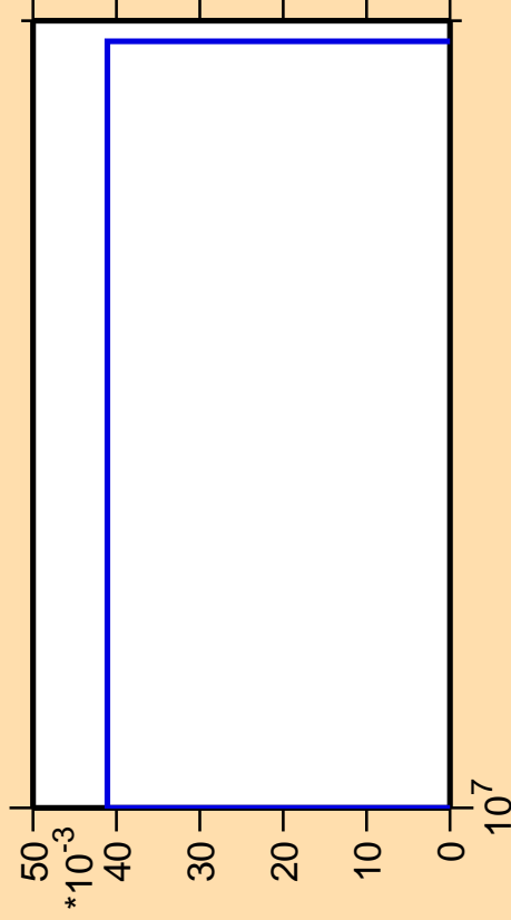
\Delta\sigma/\sigma vs. E for ^{142}\text{Nd}(n,nt)
