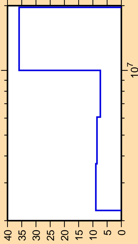
\Delta\sigma/\sigma vs. E for ^{142}\text{Nd}(n,n_{\text{cont}}) .
