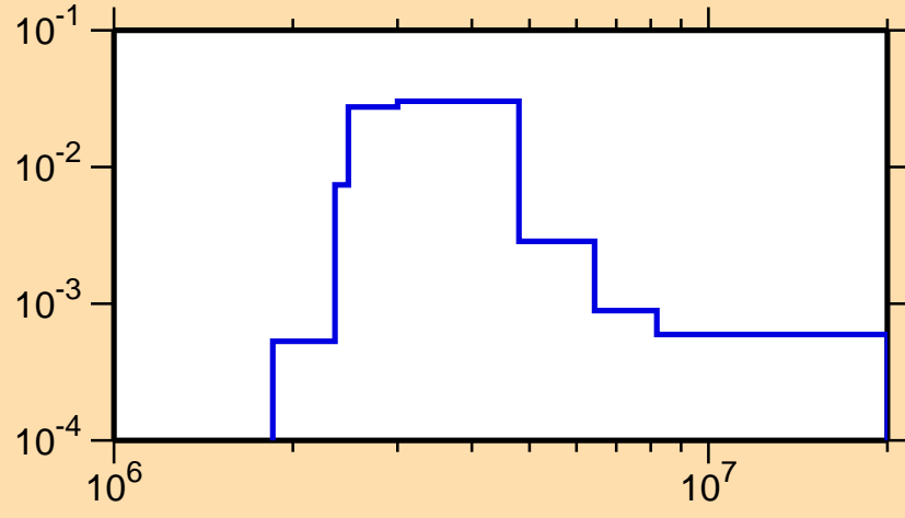
\sigma vs. E for ^{142}\text{Nd}(n,n_4)
