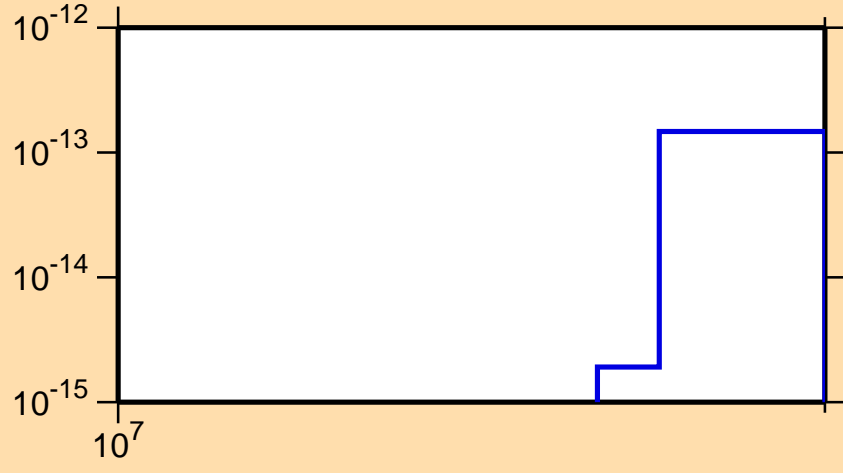
\sigma vs. E for ^{145}\text{Nd} (mt 45)
