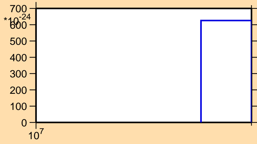
\sigma vs. E for ^{145}\text{Nd} (mt 11)
