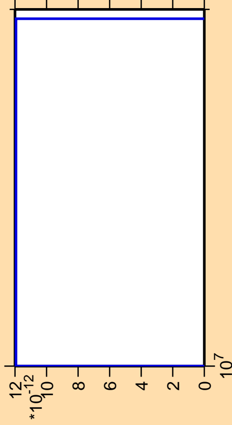
\Delta\sigma/\sigma vs. E for ^{145}\text{Nd} (mt 11)
