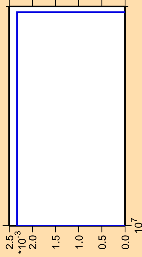
\Delta\sigma/\sigma vs. E for ^{145}\text{Nd}(n,3n\alpha)
