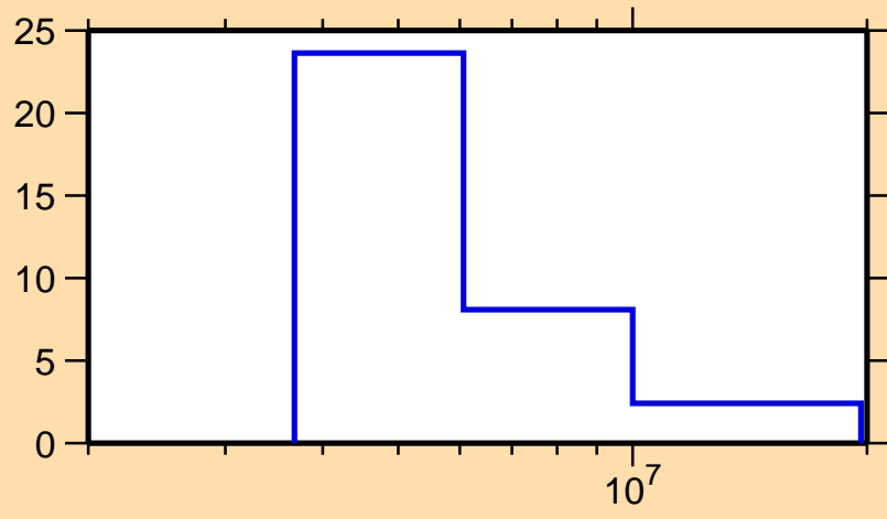
\Delta\sigma/\sigma vs. E for ^{145}\text{Nd}(n,2n)
