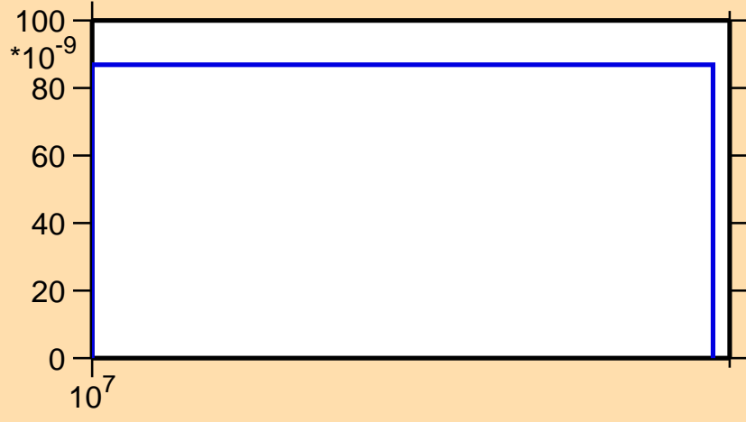
\sigma vs. E for ^{145}\text{Nd}(n,\text{nd})
