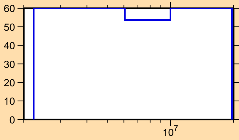
\Delta\sigma/\sigma vs. E for ^{145}\text{Nd}(n,p)
