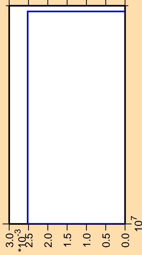
\Delta\sigma/\sigma vs. E for ^{145}\text{Nd} (mt 34)
