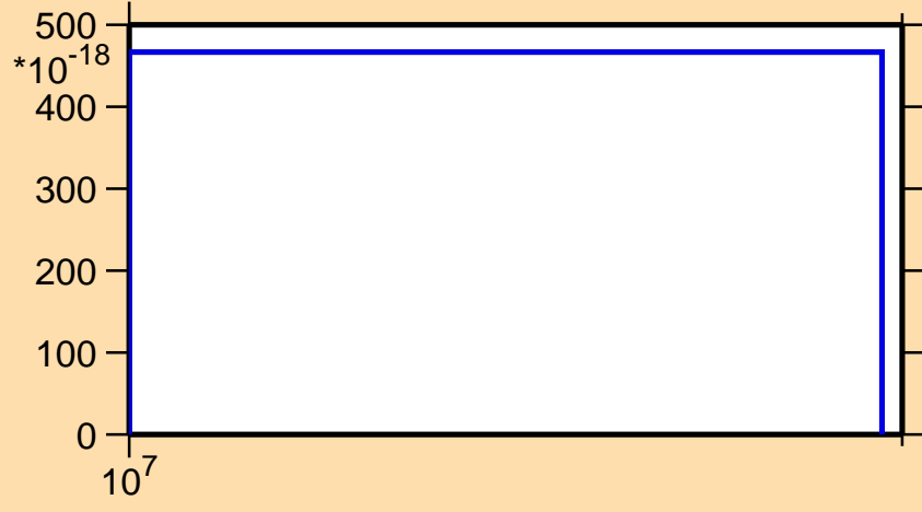
\sigma vs. E for ^{145}\text{Nd} (mt 34)
