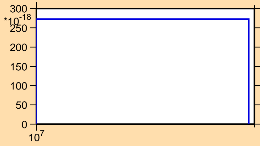
\sigma vs. E for ^{145}\text{Nd}(n,3n\alpha)
