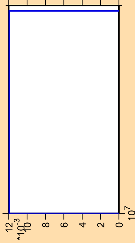
\Delta\sigma/\sigma vs. E for ^{145}\text{Nd} (mt 45)
