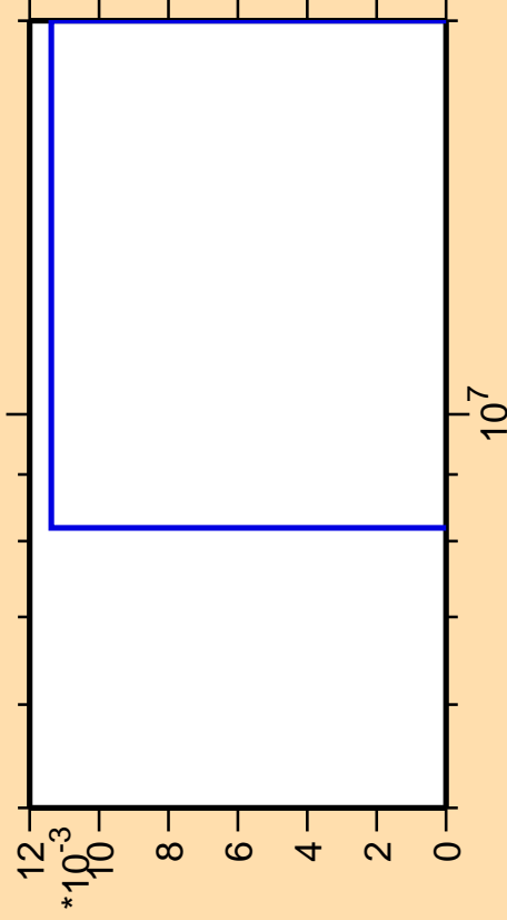
\Delta\sigma/\sigma vs. E for ^{145}\text{Nd}(\text{mt } 45)
