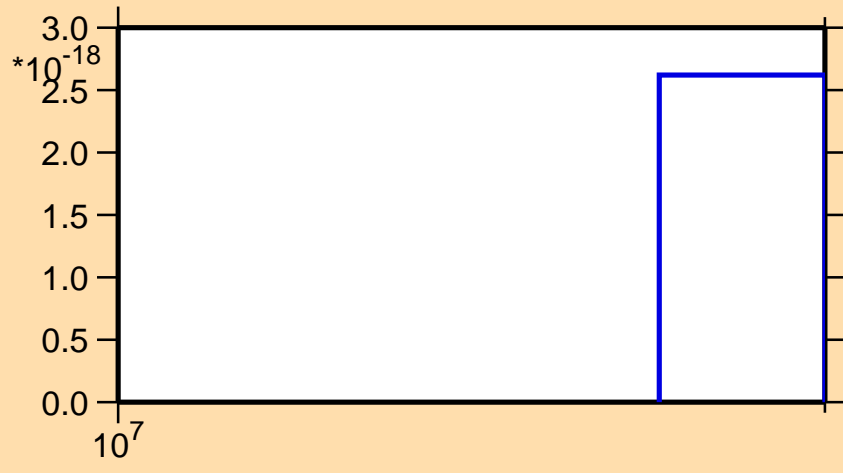
\sigma vs. E for ^{146}\text{Nd} (mt 11)
