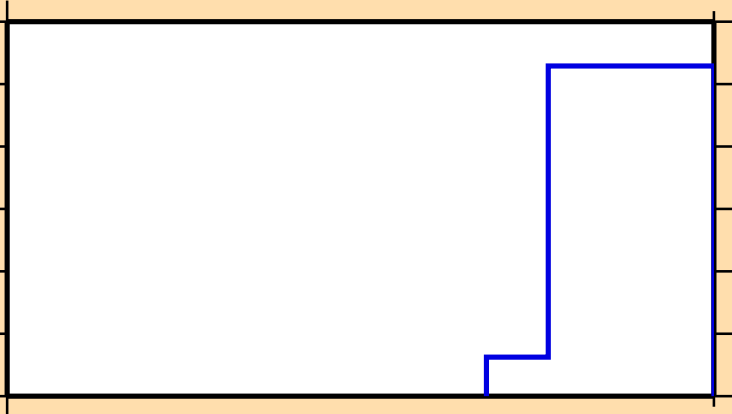
\sigma vs. E for ^{146}\text{Nd}(n,p\alpha)
