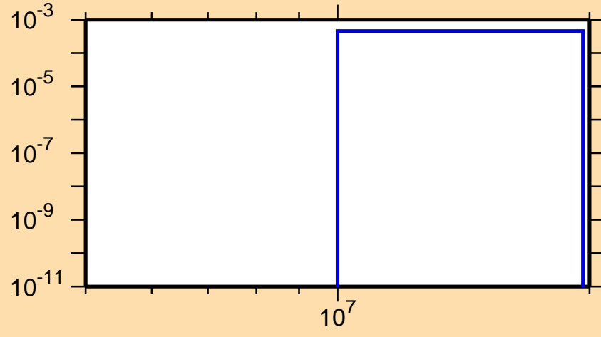
\sigma vs. E for ^{146}\text{Nd}(n,d)
