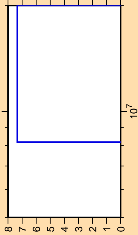
\Delta\sigma/\sigma vs. E for ^{146}\text{Nd}(n,\text{He}3)
