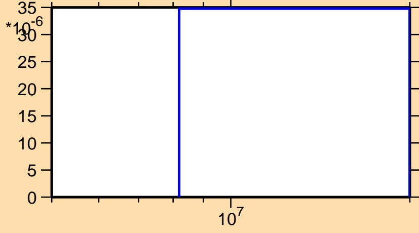
\sigma vs. E for ^{146}\text{Nd}(n,t)
