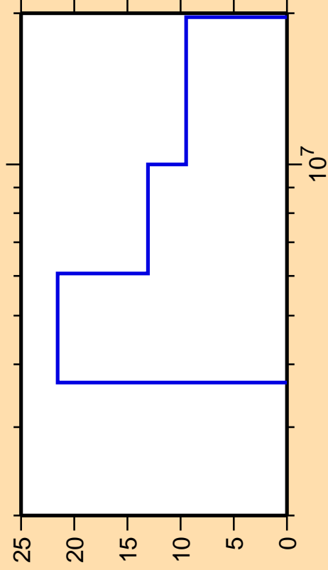
\Delta\sigma/\sigma vs. E for ^{147}\text{Nd}(n,2n)
