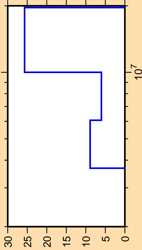
\Delta\sigma/\sigma vs. E for ^{147}\text{Nd}(n,n\text{cont.})
