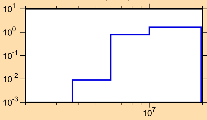
\sigma vs. E for ^{147}\text{Nd}(n,2n)
