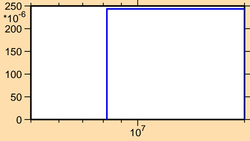
\sigma vs. E for ^{147}\text{Nd}(n,d)
