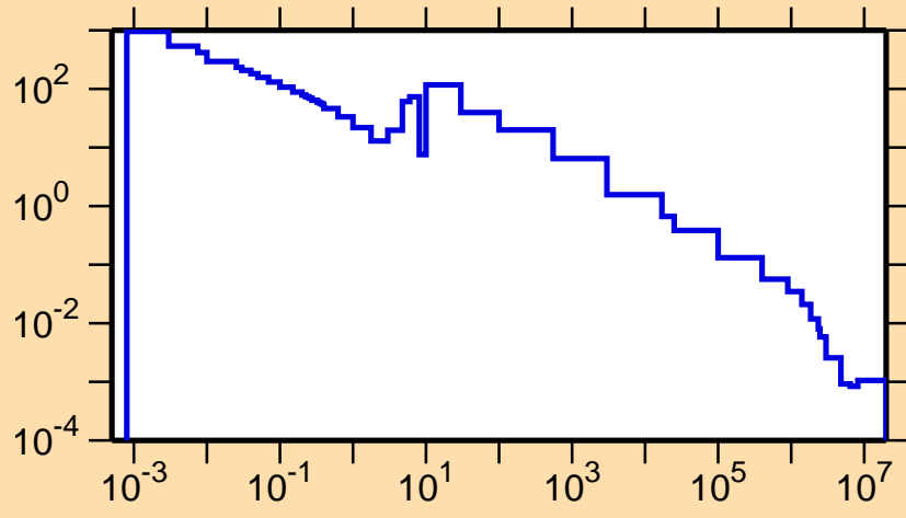
\sigma vs. E for ^{147}\text{Nd}(n,\gamma)
