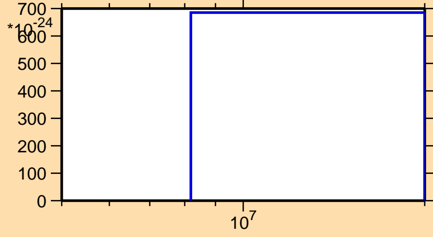
\sigma vs. E for ^{147}\text{Nd}(\text{mt } 11)
