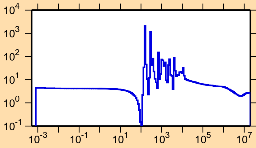
\sigma vs. E for ^{148}\text{Nd}(n,\text{el.})
